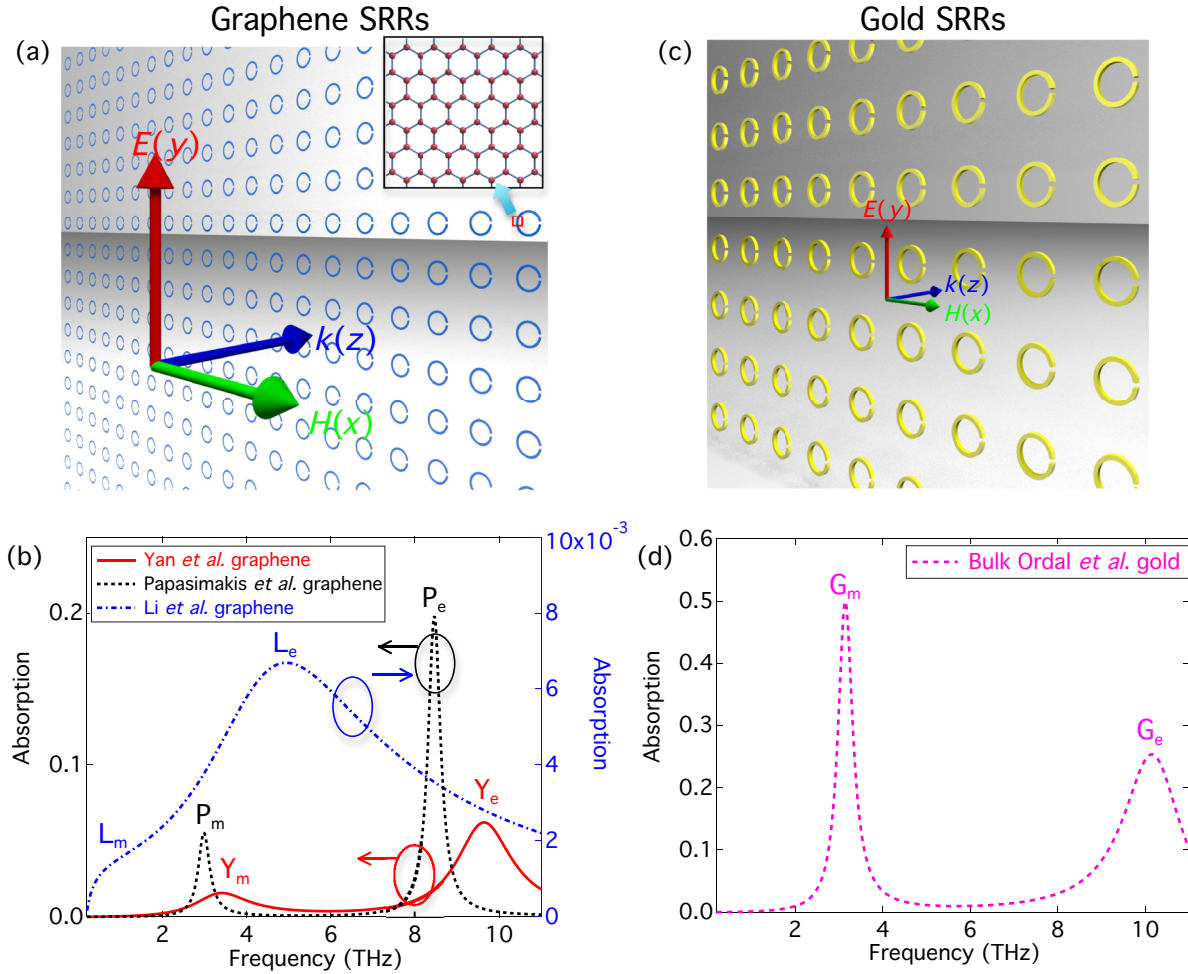
FIG. 1. (Color online) (a, b) Graphene SRRs and (c, d) gold SRRs under normal-incidence illumination. (a) Schematic diagram of graphene SRRs. Geometrical parameters are as follows: outer diameter of the ring D = 1 \mu\text{m} , ring width w = 100 \text{ nm} , gap size g = 100 \text{ nm} , and lattice constant of the graphene SRR array a = 2 \mu\text{m} . (b) Absorption spectra for SRRs made from Yan et al. [23], Papasimakis et al. [31], and Li et al. [32] graphene. (c) Schematic of 30-nm-thick gold SRRs. Geometrical parameters are outer diameter of the ring D = 15 \mu\text{m} , ring width w = 1.25 \mu\text{m} , gap size g = 1 \mu\text{m} , and lattice constant of the gold SRR array a = 25 \mu\text{m} . (d) Absorption spectrum for Ordal et al. [34] gold SRRs. The inset in (a) illustrates the honeycomb lattice of graphene.
