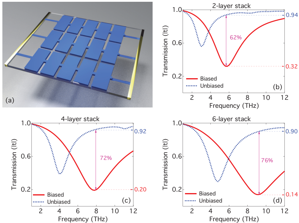
FIG. 5. (Color online) (a) Schematic of prototype of graphene THz switch with two-layer configuration: blue regions represent graphene patterns, transparent spacer is polymer and two-sided gold bars serve as contact for odd and even graphene layer(s), respectively. (b)–(d) show the performance in transmission for switching on/off through biased/unbiased patterned graphene stack with two, four, and six layers.
