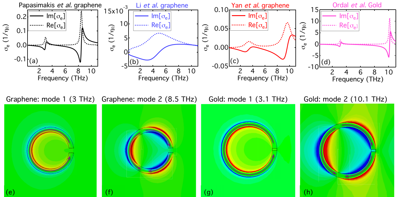
FIG. 2. (Color online) Retrieved frequency-dependent electric sheet conductivity (upper row) and z -component magnetic field distributions (lower row) for graphene and gold SRRs under normal incidence, respectively. (e) and (f) corresponds two modes for Papasimakis et al. graphene case; (g) and (h) are for case of Ordal et al. gold SRRs. Arrows in (e)–(h) give the direction of currents.
