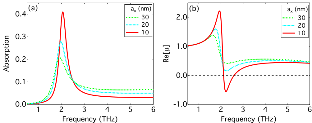
FIG. 4. (Color online) (a) Absorption spectra and (b) effective permeability for Yan et al. graphene SRRs under parallel incidence with a_x = 10, 20, 30 \text{ nm} .
