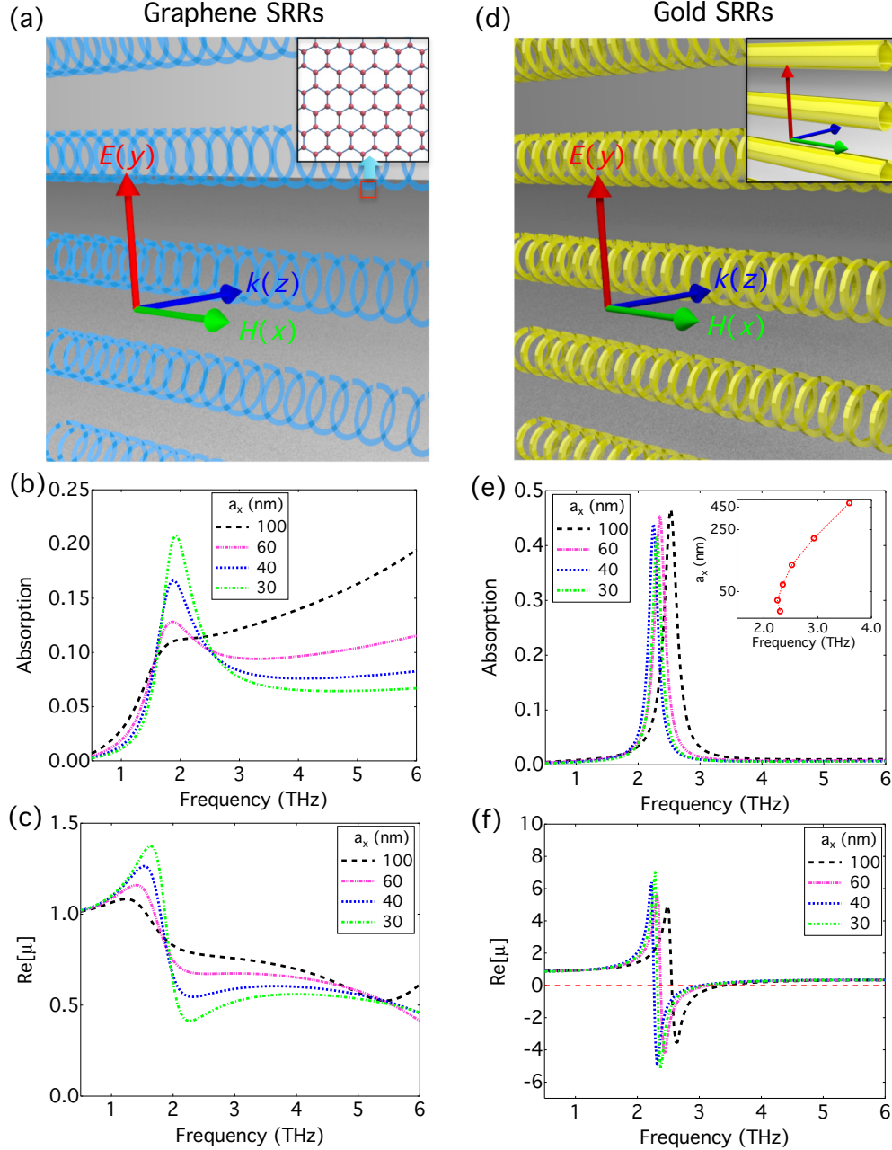
FIG. 3. (Color online) (a)–(c) Graphene SRRs and (d)–(f) gold SRRs under parallel-incidence illumination. (a, d) Schematics of the geometries. Geometric parameters are outer diameter of the ring D = 5 \mu\text{m} , ring width w = 500 \text{ nm} , gap size g = 500 \text{ nm} , and in-plane lattice constant a = 6 \mu\text{m} . (b) Absorption spectra and (c) effective parameter \text{Re}[\mu] for SRRs made from Yan et al. graphene with different ring separations a_x : 100, 60, 40, and 30 nm. (e) Absorption spectra and (f) effective parameter \text{Re}[\mu] for Ordal et al. gold SRRs. The inset in (e) illustrates resonance frequency in dependence of ring separation a_x for gold SRRs.
