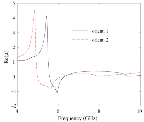
Fig. 6. Simulation results for the real part of the effective permeability, \mu , of our SRR system, as obtained from the theoretical transmission and reflection data, through the standard retrieval procedure.
