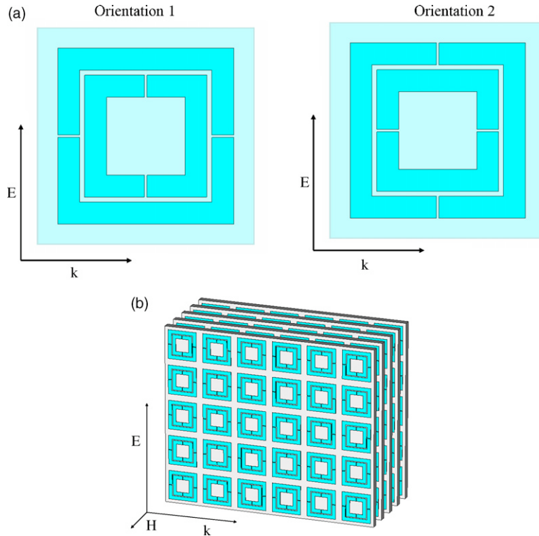
Fig. 2. (a) The unit cell of the proposed double ring design with two cuts per ring, for two orientations with respect to the incoming electromagnetic field, characterized by the wave vector, \mathbf{k} , the electric field, \mathbf{E} , and the magnetic field, \mathbf{H} (perpendicular to the plane of (\mathbf{E}, \mathbf{k}) —not shown here). The system parameters are as follows: unit cell size along \mathbf{E} and \mathbf{k} axes is 8.8 mm, SRR linear size = 7.2 mm, rings' width = 0.9 mm, gaps width = 0.1 mm, rings distance in the double ring = 0.2 mm, metal thickness = 30 \mu\text{m} . The board where the SRRs are printed is FR-4, with thickness 1.6 mm. (b) The periodic arrangement of our SRRs.
