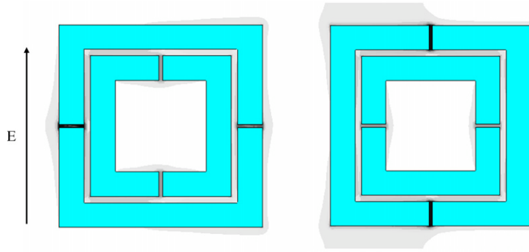
Fig. 4. The size of the electric field ( |E| ) at the magnetic resonance frequency shown in Fig. 3. Left panel shows the field for orientation 1 and right panel for orientation 2. Dark (light) color indicates high (low) field values. For orientation 2 the field between the inner and the outer ring is stronger than in orientation 1, as well as the field among neighboring unit cells along the E direction, indicating a larger effective capacitance and, hence, a lower resonance frequency (assuming that the effective inductance is about the same).
