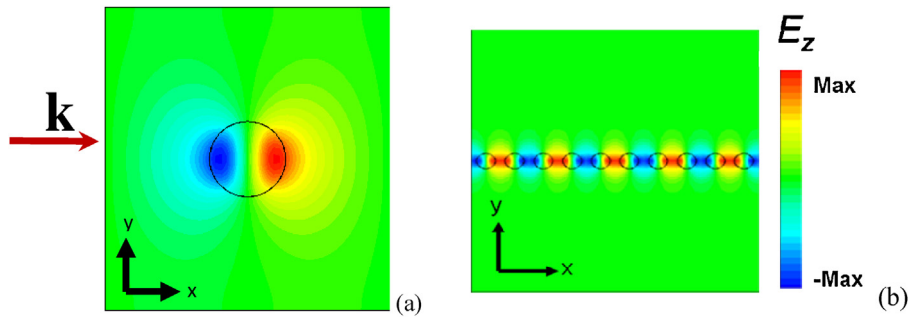
Fig. 6. (a) The scattered electric field by a dielectric cylinder (of relative permittivity 40 and radius 4\ \mu\text{m} ) embedded in an ENZ medium at the region of a cylinder resonance (4.54 THz). The electric field in the incoming wave is parallel to the cylinder. (b) Very confined almost perfect propagation along an array of dielectric cylinders (as the one shown in panel (a)) embedded in an ENZ medium due to the p-like symmetry of each individual scattered field. The guiding occurs at frequency 4.55 THz, i.e. almost identical to the frequency of a Mie-resonance.
