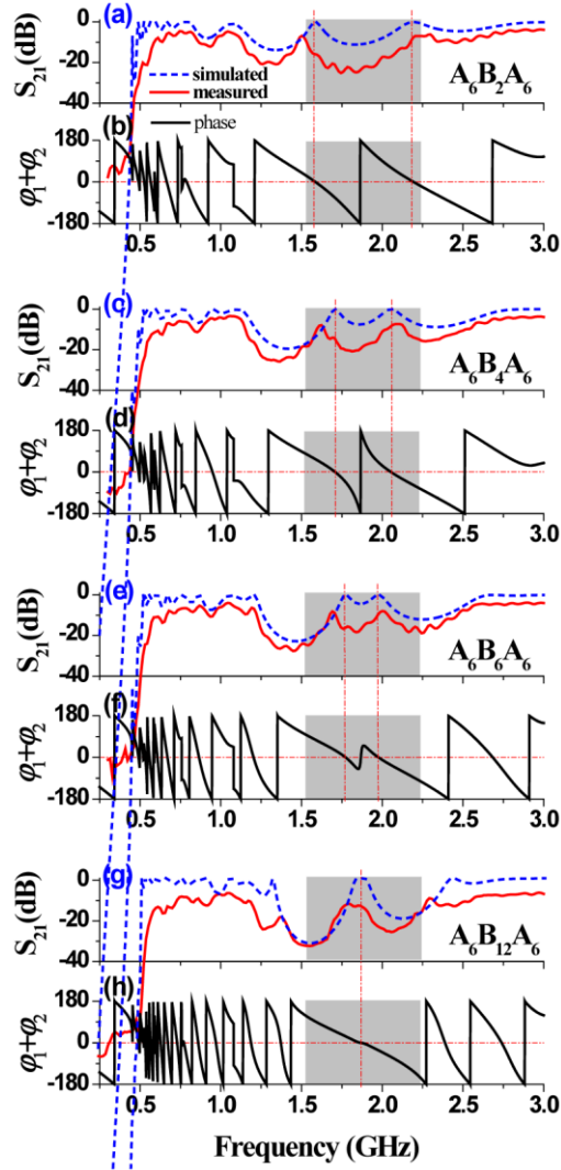
Fig. 8. The simulated and measured S_{21} parameters and the simulated values of \phi_1(\omega) + \phi_2(\omega) for SNG sandwich structures A_6B_2A_6 (a & b), A_6B_4A_6 (c & d), A_6B_6A_6 (e & f) and A_6B_{12}A_6 (g & h), respectively. The grey regions correspond to the common SNG frequency range of TLs A and B.
