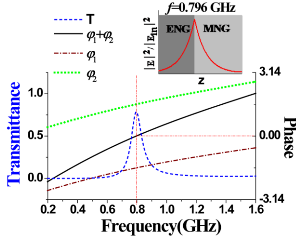
Fig. 2. Transmittance and phase changes as a function of frequency for pair SNG structures. The thicknesses of the ENG and MNG layers are 30 nm and 40 nm, respectively. The inset shows the electric field distribution at 0.796 GHz.
