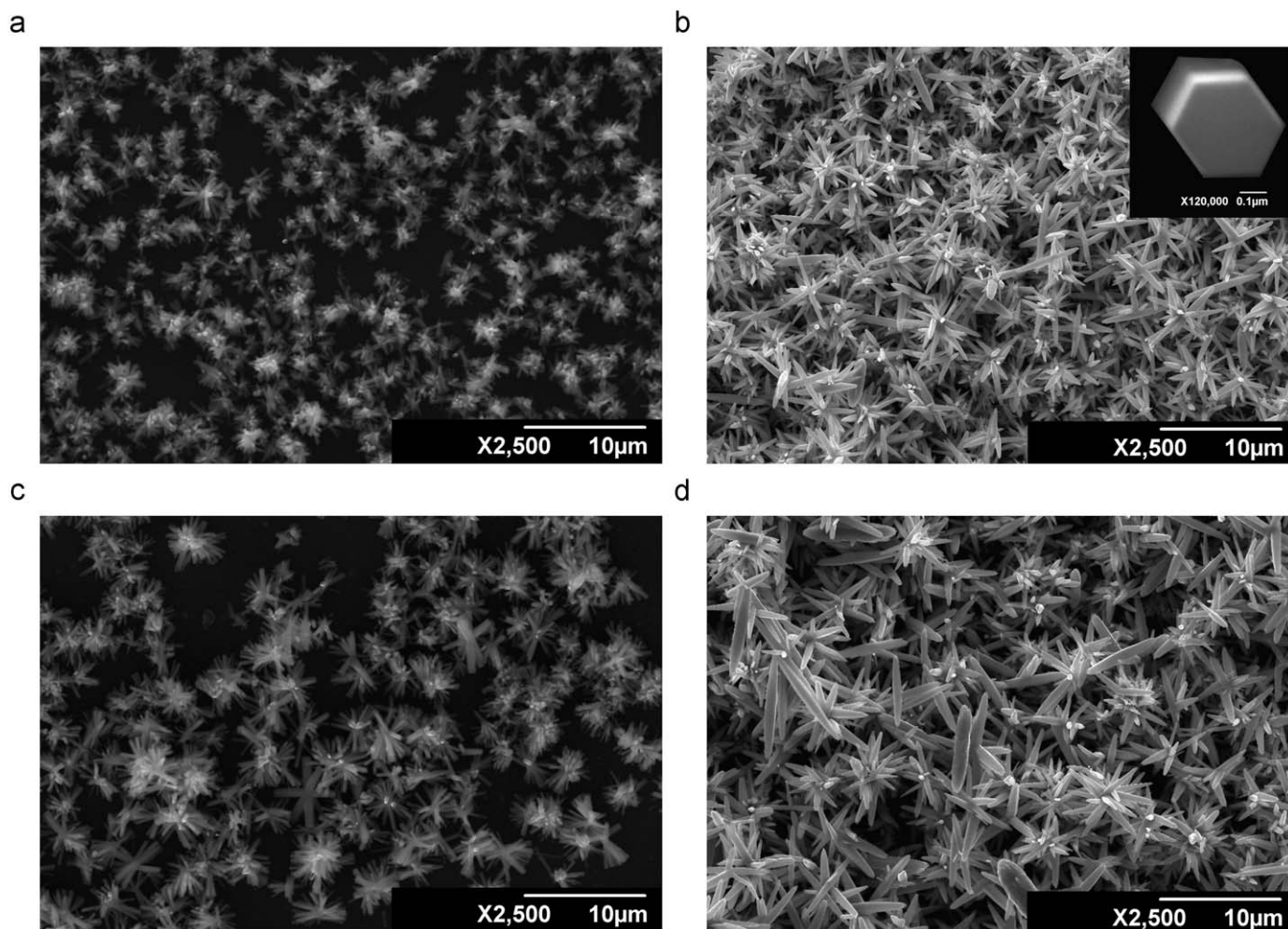
Fig. 2. SEM images of ZnO nanostructures grown by aqueous solution growth on bare Corning glass substrates for (a) 2 h and (b) 5 h, and on bare silicon (100) substrates for (c) 2 h and (d) 5 h. In the inset of (b) the hexagonal cross section of the ZnO nanorods is clearly observed.
