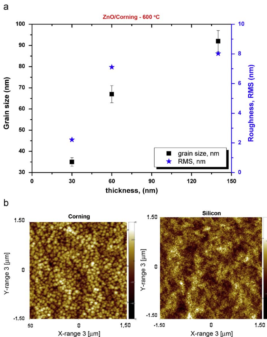
Fig. 4. (a) Grain size (black squares) and roughness (blue stars) vs. thickness of the sol-gel deposited ZnO seed layers on Corning glass annealed at 600 °C and (b) AFM images (scan size 3 μm × 3 μm) of 140-nm-thick ZnO seed layers on Corning (left) and silicon (right) substrates. (For interpretation of the references to colour in this figure legend, the reader is referred to the web version of this article.)
