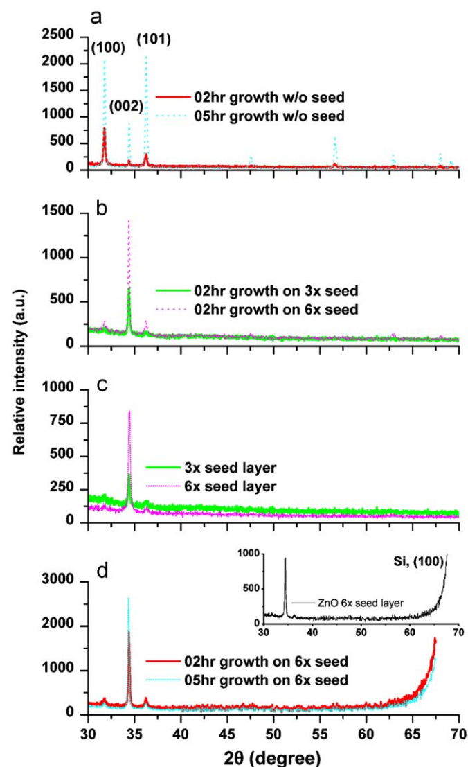
Fig. 1. XRD patterns of (a) ZnO samples grown by aqueous solution growth on bare Corning glass substrates for 2 h (red curve) and 5 h (light-blue dashed curve), (b) ZnO samples grown by aqueous solution growth for 2 h on Corning glass substrates with a 3-layered (60-nm-thick, green curve) and a 6-layered (140-nm-thick, magenta dashed curve) ZnO seed layer, (c) 3-layered (60-nm-thick, green curve) and 6-layered (140-nm-thick, magenta dashed curve) ZnO seed layers deposited via sol-gel on Corning glass substrates, and (d) ZnO samples grown by aqueous solution growth on silicon (100) substrates with a 6-layered (140-nm-thick) ZnO seed layer for 2 h (red curve) and 5 h (light-blue dashed curve). In the inset of (d) the XRD pattern of a 6-layered (140-nm-thick) ZnO seed layer deposited on Si (100) via sol-gel is presented. (For interpretation of the references to colour in this figure legend, the reader is referred to the web version of this article.)
