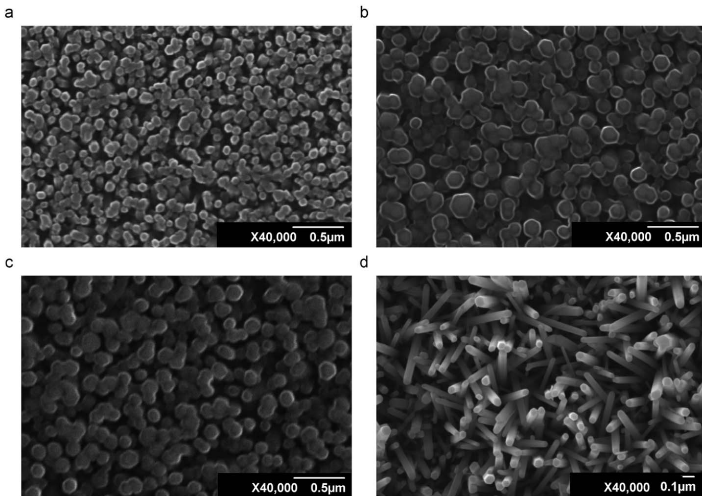
Fig. 3. SEM images of ZnO nanowires grown by aqueous solution growth for (a) 2 h on Corning glass/60-nm-thick ZnO seed layer, (b) 2 h on Corning glass/140-nm-thick ZnO seed layer, (c) 5 h on Corning glass/140-nm-thick ZnO seed layer and (d) 5 h on silicon (100)/140-nm-thick ZnO seed layer.
