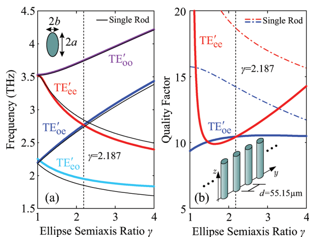
Figure 3. Metasurface made of elliptical rods with a pitch d = 55.15 \mu m . Evolution of TE-polarization collective resonances as the eccentricity varies. a) Resonant frequencies and b) quality factors as a function of the semiaxis ratio \gamma = a/b . TE'_{oe} (MD) and TE'_{ee} (TD) resonances match in frequency and quality factor for \gamma = 2.187 .
