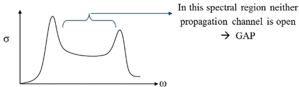
FIG. 4. Schematic plot of a typical behavior of the scattering cross-section by a single inclusion vs frequency for the case where the inclusion mass density is much higher than that of the host and their sound velocities are of the same order of magnitude.
