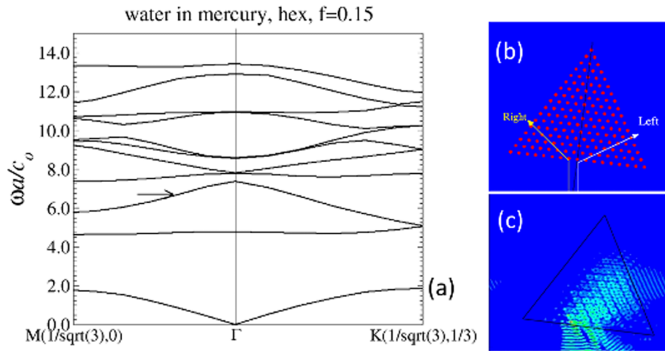
FIG. 9. (a): The band structure of a periodic acoustic system made of water cylinders in mercury in hexagonal; arrangement. Here a is the lattice constant. The cylinder volume fraction is 15%. The band marked by the arrow has negative curvature which indicates opposite phase and group velocity and therefore left-handed behavior and negative refraction (see, e.g., Ref. 28). This negative refraction response is demonstrated in panel (c), where a wave (of dimensionless frequency 7) impinges on a prism-shaped phononic crystal like the one shown in panel (b). In the above calculations the mercury parameters employed are \rho=13500 \text{ kgr/m}^3 , c_l=1531 \text{ m/s} and the water ones \rho = 1025 \text{ kgr/m}^3 , c_l = 1450 \text{ m/s} .
