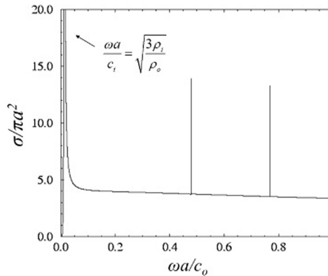
FIG. 7. Dimensionless scattering cross-section by a spherical air bubble of radius a in water as a function of the dimensionless frequency \omega a/c_0 , where c_0 is the sound velocity in water. Notice the very strong resonance at low frequency (Minnaert resonance) due to the uniform compression of the bubble.
