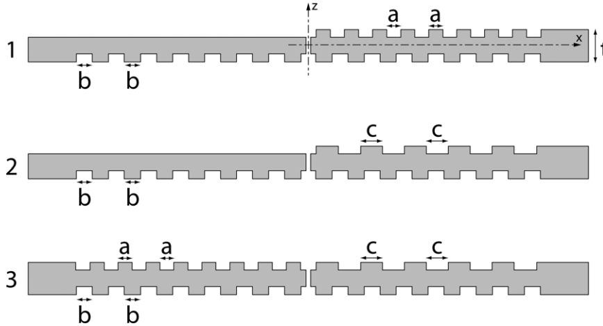
Figure 1. The structures used in this work were a = 7 mm, b = 8 mm, c = 11 mm and t = 16 mm. The slit widths were 2 mm and the grating heights were 4 mm. All of them had the same input surface grating period of 16 mm in order to couple the ‘spoof’ surface plasmons.
