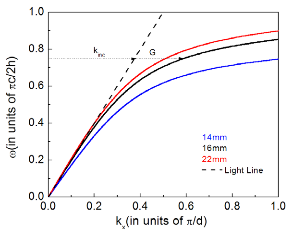
Figure 6. The dispersion relation of the surface modes supported by metallic structures with grooves of periods 14 mm (blue line), 16 mm (black line) and 22 mm (red line). The light line is shown with a dashed line. (Colour online.)
