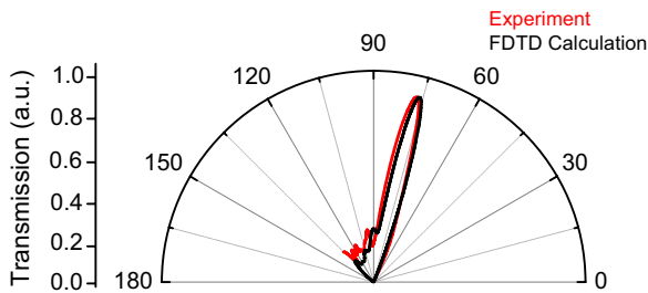
Figure 4. By use of a metallic structure with a subwavelength aperture at the centre and the grating periods of 14 mm and 22 mm on the different sides of the output surface, we observed off-axis directional beaming with an FWHM of 10° and the beaming angle of 15°. It is possible to steer the beaming angle by arranging the grating periods of the output surface of the metallic structure.
