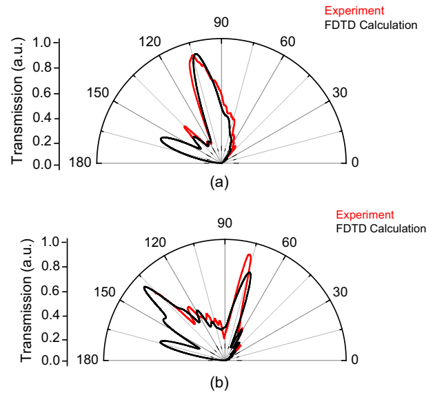
Figure 2. The beaming angle is steered for structures with grating periods only on one side of the output surface. The beam is mostly directed to the negative side for (a) Sample 1 and positive side for (b) Sample 2 at 14.5 GHz (20.7 mm).
