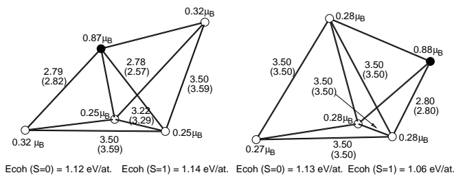
Fig. 2. Electronic and structural properties of the calculated isomers of \text{NiNa}_4 . Filled (open) circles indicate Ni (Na) atoms. Results are given for the cohesive energy per atom E_{coh} , nearest neighbor bond-lengths (in Å), and local magnetic moments \mu(i) in the magnetic solution having z component of the total spin S_z = 1 . The values in brackets refer to the non-magnetic solution.
