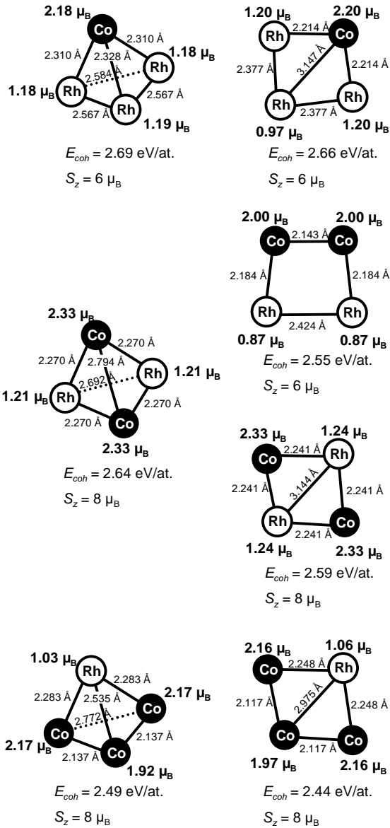
Fig. 1. Magnetic and structural properties of \text{Co}_M\text{Rh}_N clusters having N+M=4 atoms. Results are given for the cohesive energy per atom E_{coh} , nearest-neighbor bond-lengths, z component S_z of the total spin moment, and local spin moments \mu(i) at each atom i .
