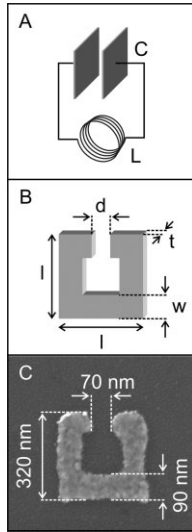
Figure 9. Illustration of the analogy between a usual LC circuit (A) and a SRR (B). C) Electron microscopy image of a fabricated structure, a gold SRR (metal thickness t=20 nm) on a glass substrate. Reprinted with permission from [20]. Copyright 2004 American Association for the Advancement of Science.
